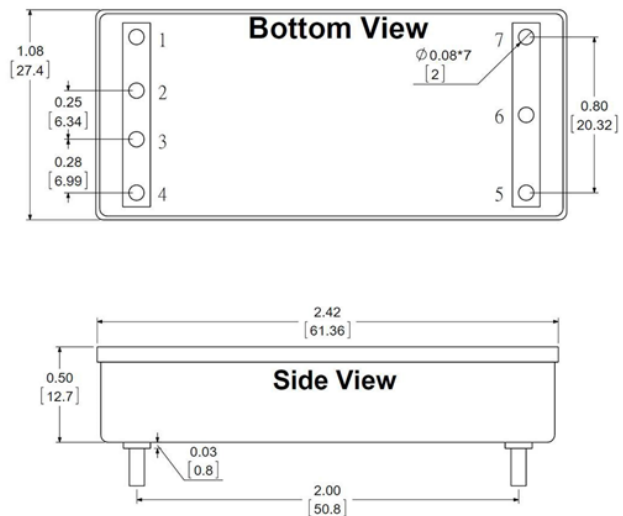
Shape – F (No Flange Base Plate with Vicor pinout)
